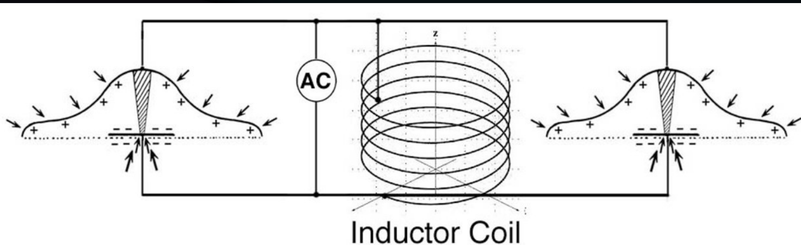
Figure 140. Tank circuit configuration of Brown's asymmetrical capacitor electrokinetic thrusters allowing them to repeatedly charge and discharge with a minimal of input power. Arrows indicate the direction of the electrostatic forces. Upward forces would dominate due to the stronger field intensity on the negative electrode.
